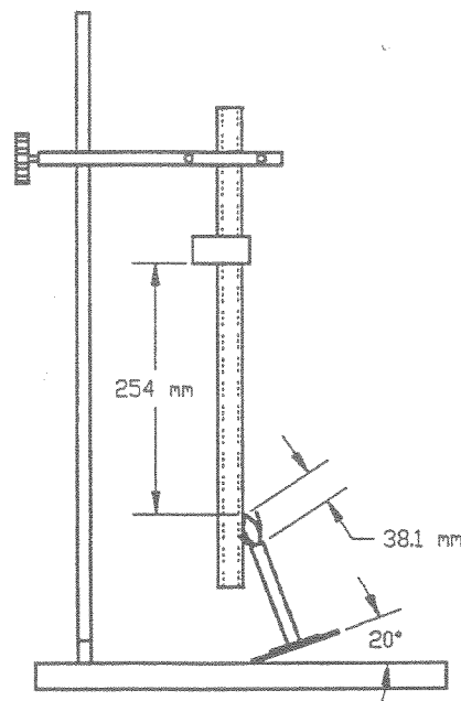
Figure 1—Test apparatus
